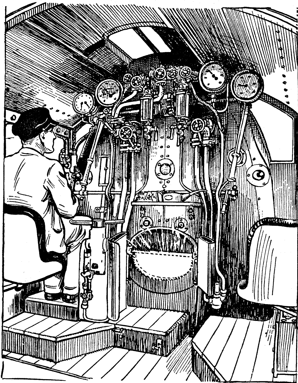
With the driver in the cab of a streamlined Pacific. The firehole is open for the fireman to throw coal into the firebox.
